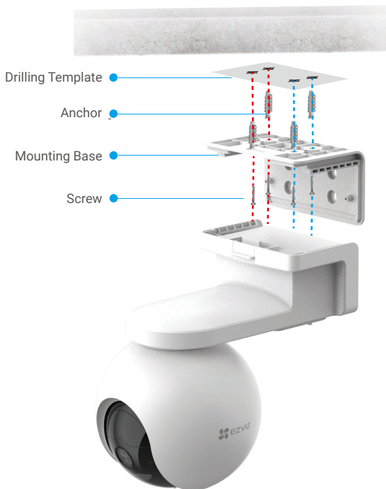
Fig. 1 Ceiling Mount
